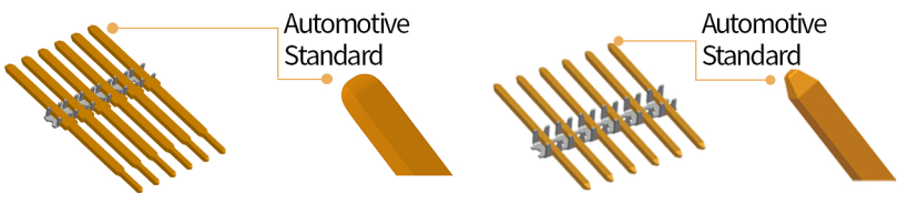
Spring-Clip Terminals
